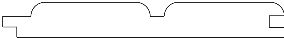
OTG-8014 5/8" x 4-1/2" FACE
