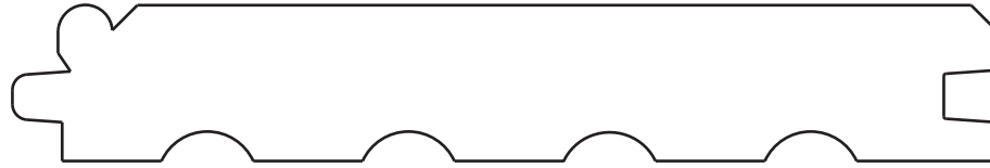
OTG-8008 3/4" x 4-1/2" FACE
